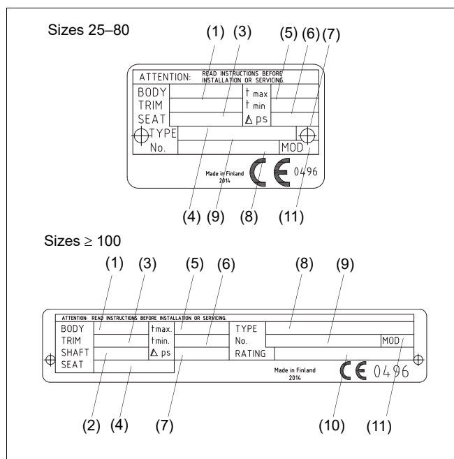
Fig. 3 Identification plate
