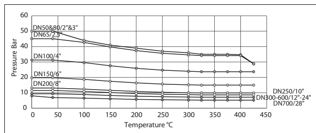
Fig. 9 Max operating pressure differential in control service, Q-RE opening range 30 %-60 %
