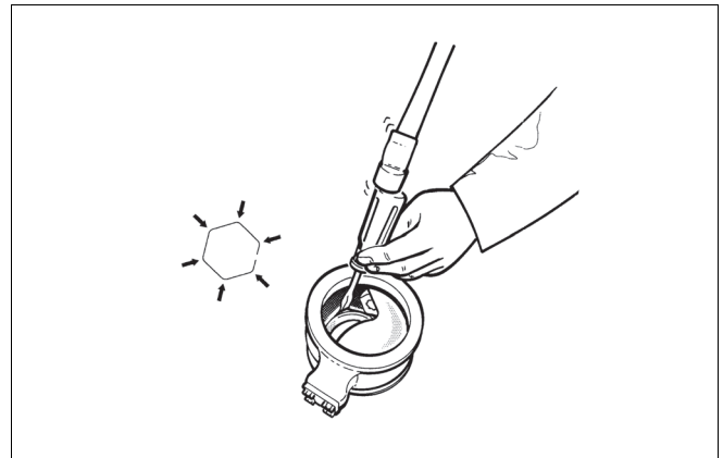
Fig. 29 Knocking the spring into the groove
