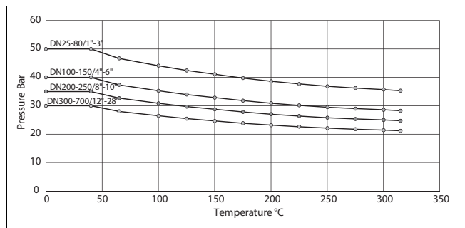
Fig. 11 Maximum pressure differentials in on-off operation, AISI 329 Shaft
